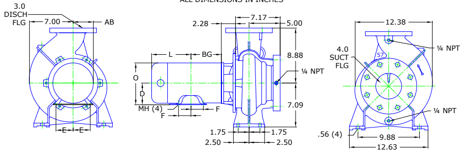
DRAWING DEPICTS JM145 1HP ODP MOTOR ALL DIMENSIONS IN INCHES
