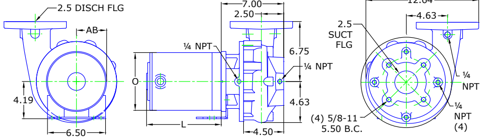
DRAWING DEPICTS 56C ODP MOTOR ALL DIMENSIONS IN INCHES
