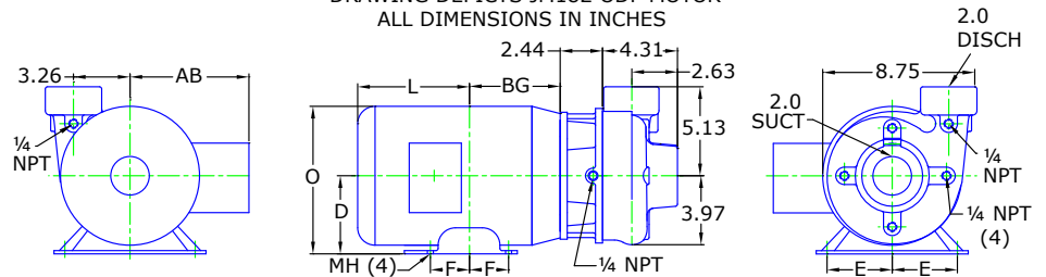
DRAWING DEPICTS JM182 ODP MOTOR ALL DIMENSIONS IN INCHES
