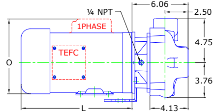
DRAWING DEPICTS 56J 1PHASE TEFC MOTOR ALL DIMENSIONS IN INCHES
